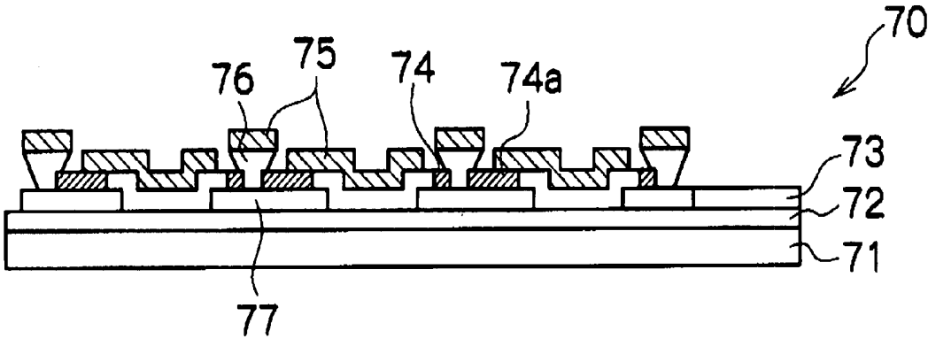
A-A' CROSS-SECTION
